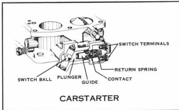
STARTER SWITCH (certain models only)
