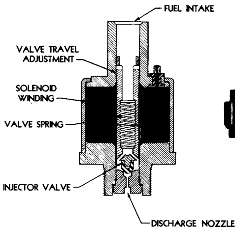
FIG. 2 THE FUEL INJECTOR
