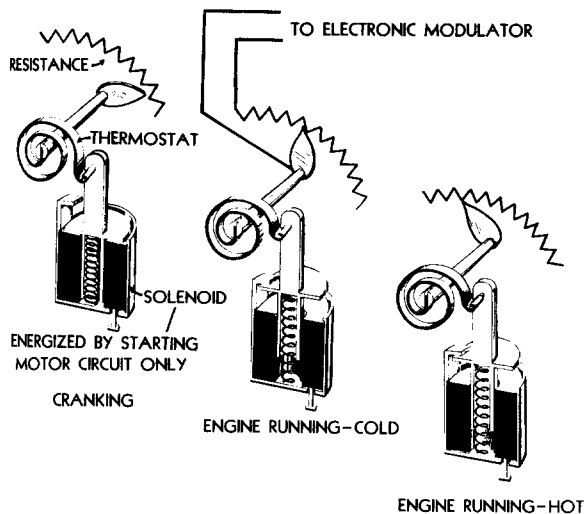
FIG. 10 STARTING ENRICHMENT
