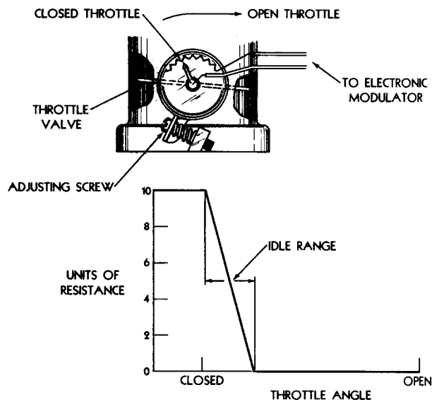
FIG. 9 IDLE ENRICHMENT
